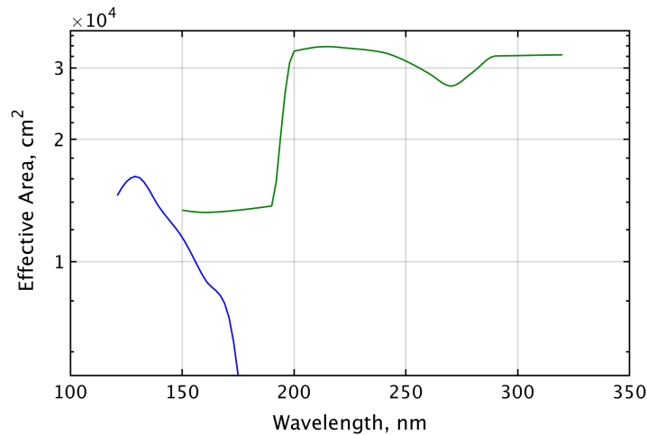
Figure 7: Effective area of the FCU
